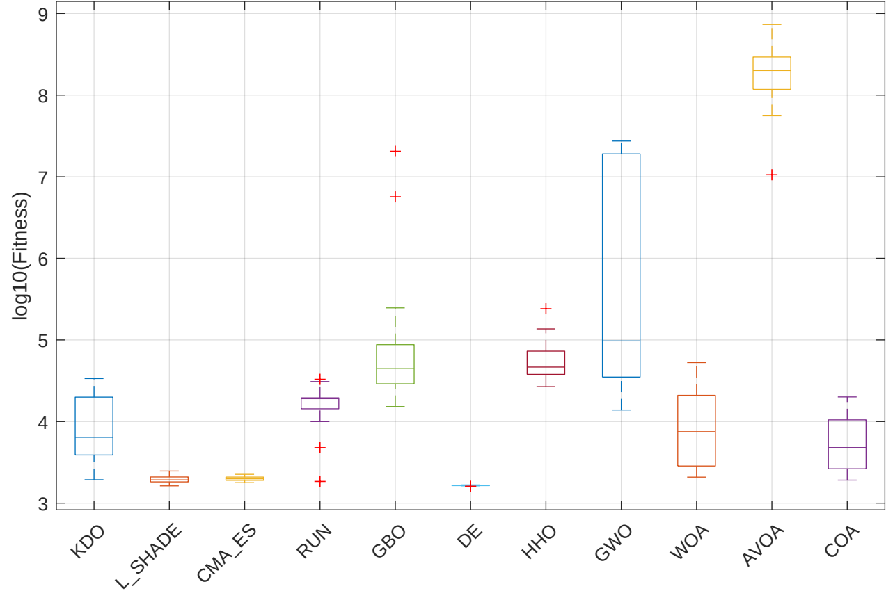
CEC2017 F15 (Numerical) - Boxplot
